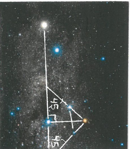
ALPHA CENTAURI (AT LEFT) AND THE SOUTHERN CROSS. 2nd ALPHA CENTAURI IS THE CLOSEST SUN TO OURS. IT HAS SAME DIAMETER AS OURS, AND IS 4.3 LIGHTYEARS AWAY
