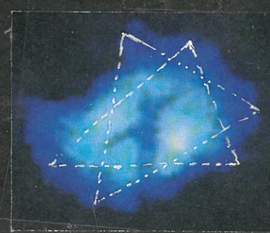
Whirlpool Galaxy center black-hole
