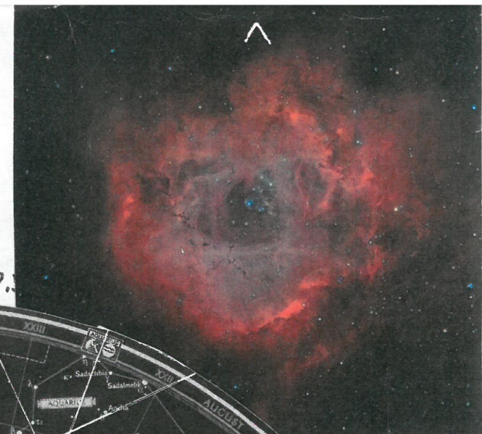
Rosette Nebula
