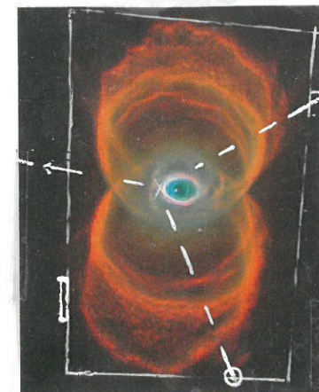
Hourglass Nebula with Temple Mosque footprint
