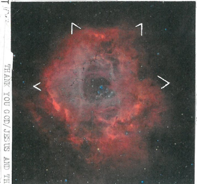
ROSETTE NEBULA
