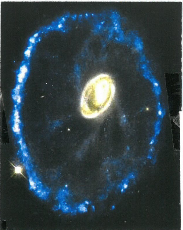
CARTWHEEL GALAXY
